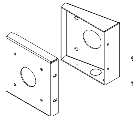
AUXILIARY VIEW
